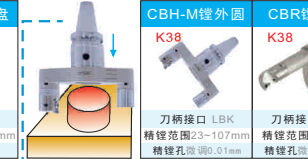
镗外圆 Boring Outer Circle
